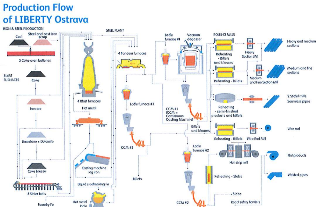
Fig. 1: Production Process Flow Diagram
