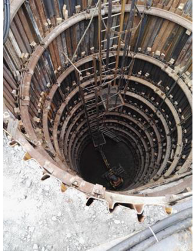
Combined use of casing profiles UNION with mining support arches on the construction of one collector.
