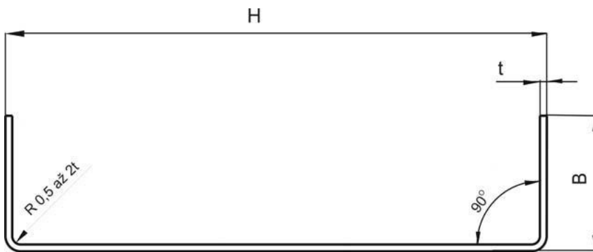
U-Profiles
